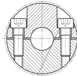
Splitnav
